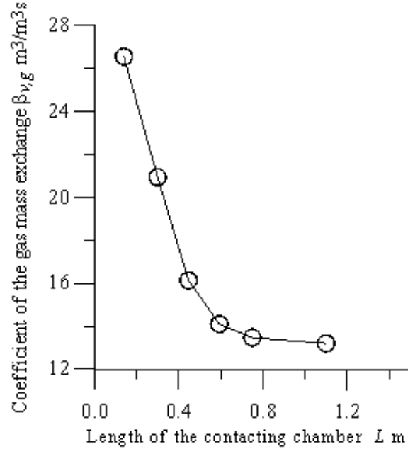
Figure 4: Coefficient of the gas mass exchange \beta_{v,g} versus height of the contacting chamber L_{cont} .
