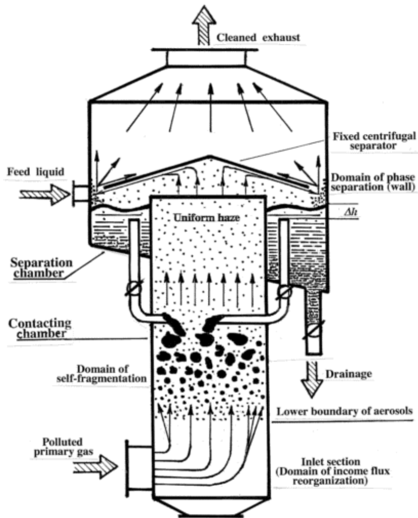
Figure 1: Schematic diagram of one-stage Low Speed Absorber (LSA).
