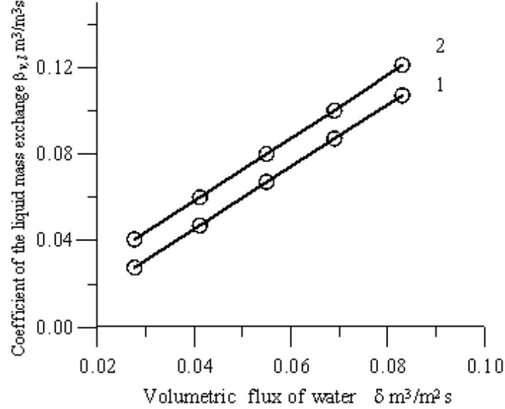
Figure 3: Coefficient of the liquid mass exchange \beta_{v,l} versus volumetric flux of water \delta , 1- u=10 m/s, 2- u=20 m/s.
