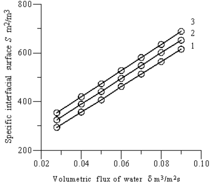
Figure 2: Specific interfacial surface S versus volumetric flux of water \delta , 1- u= 10 m/s, 2- u= 15 m/s, 3- u= 20 m/s.
